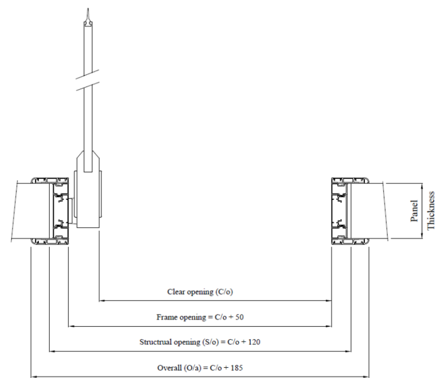
Single Leaf Door
